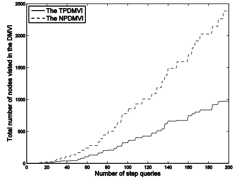
Fig. 9. The performance of the view searching with invalid search paths between the TPDMVI and the NPDMVI
